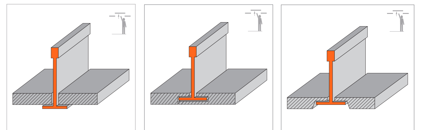
PERFIL VISTO EXPOSED FORM
