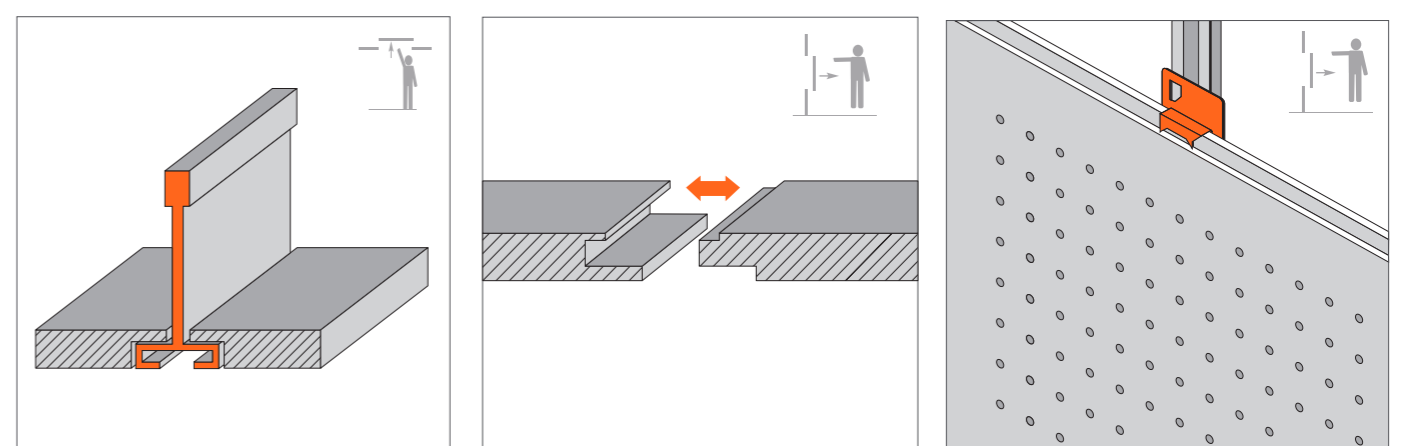
PERFIL FINLINE T-15 FINLINE FORM T-15
